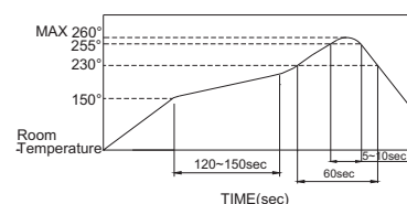
Reflow Temperature Profile:
